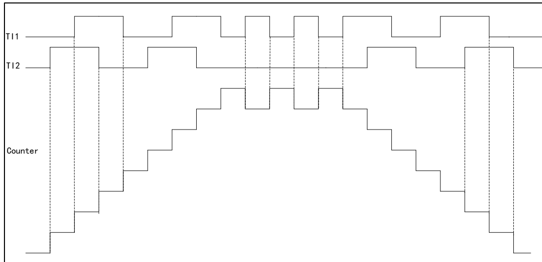
Figure 55 Counter Operation Example in Encoder Mode
