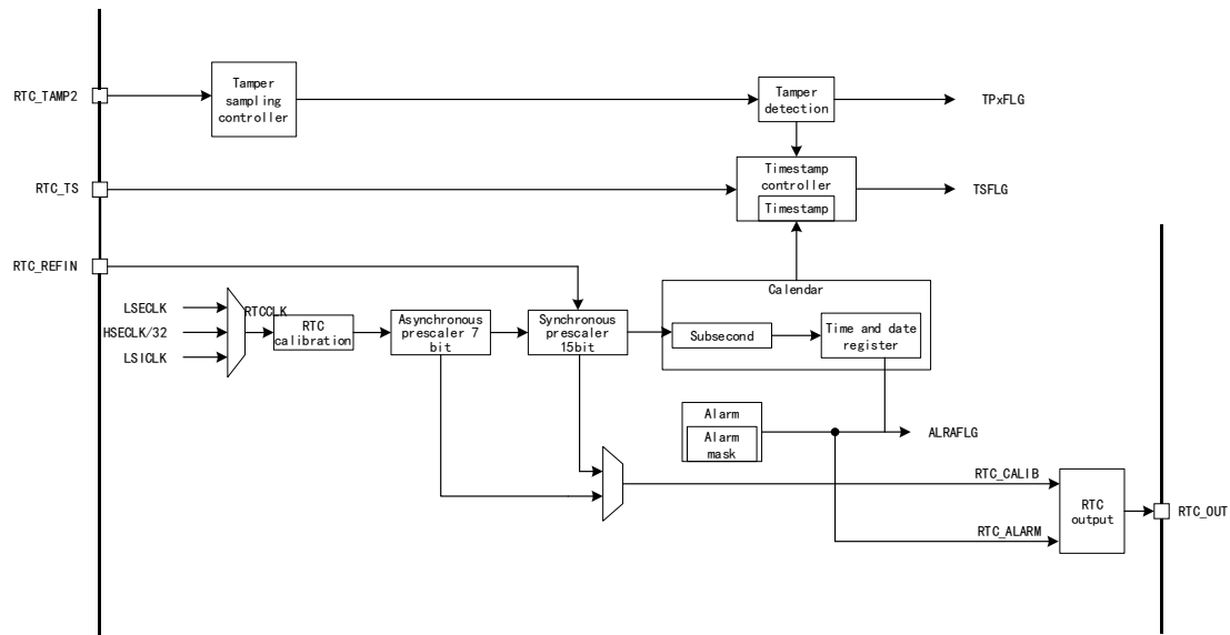
Figure 82 RTC Structure Block Diagram
