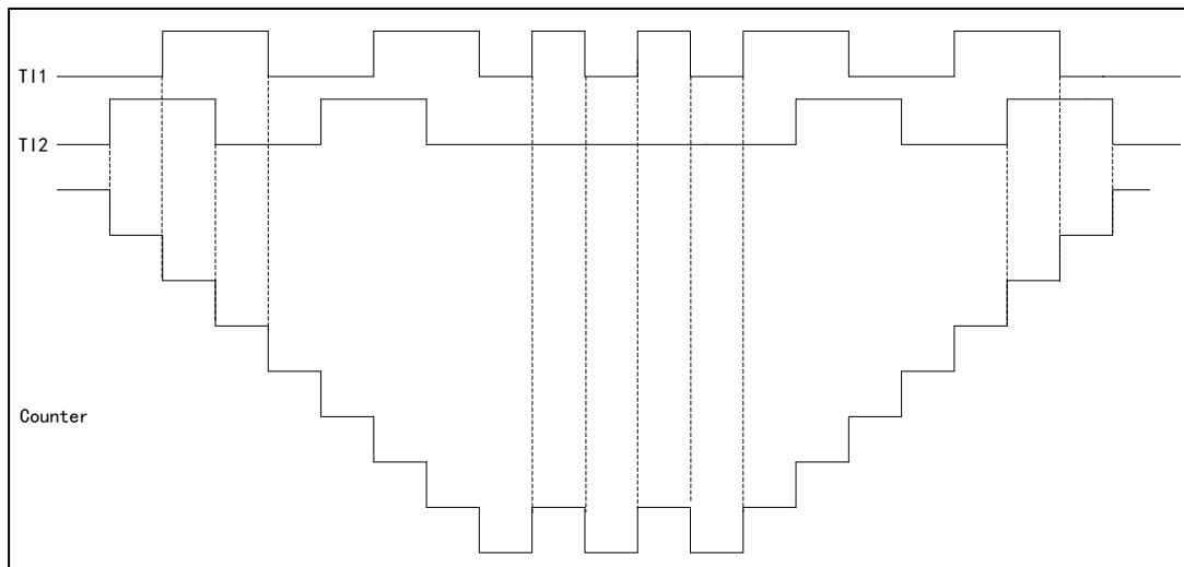
Figure 56 Example of Encoder Interface Mode of TI1FP1 Reversed Phase
