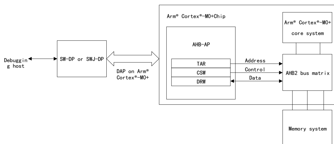
Figure 15 APM32E0xx Level and Arm® Cortex®-M0+ Level Debugging Block Diagram
