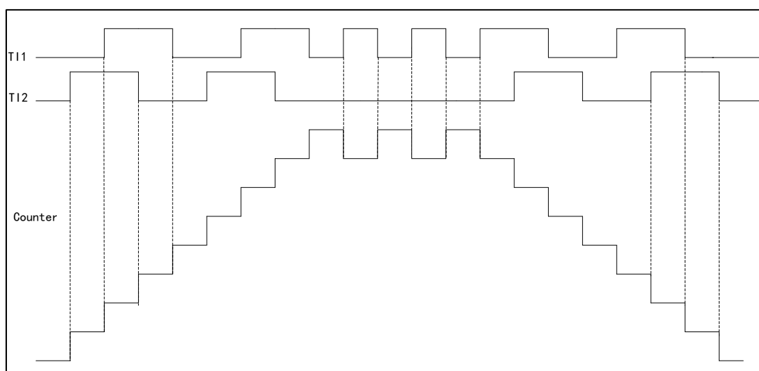
Figure 38 Counter Operation Example in Encoder Mode
