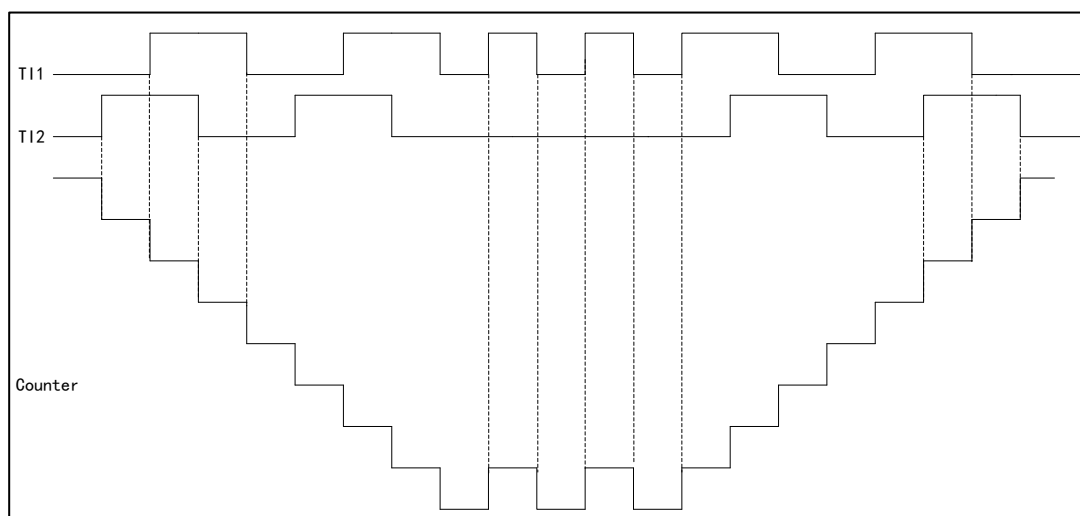
Figure 39 Example of Encoder Interface Mode of TI1FP1 Reversed Phase
