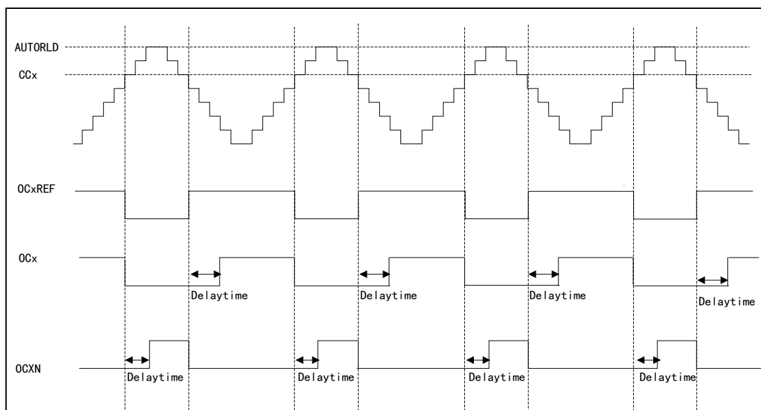
Figure 37 Complementary Output of Insertion with Dead-time
