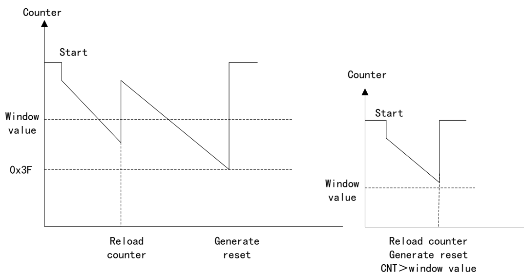
Figure 81 Window Watchdog Timing Diagram
